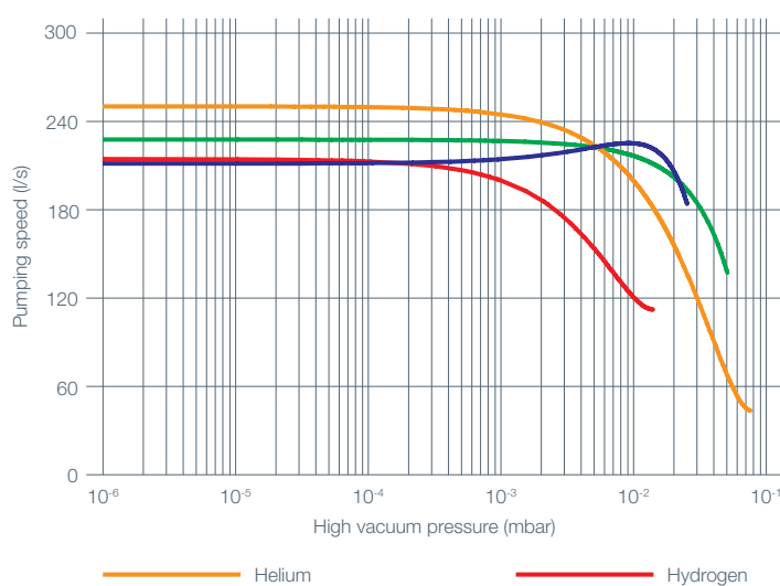
TURBOVAC 250 i/iX
