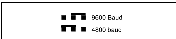
W7 Jumper
