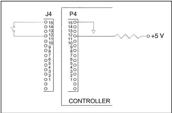
Typical Logic Input
