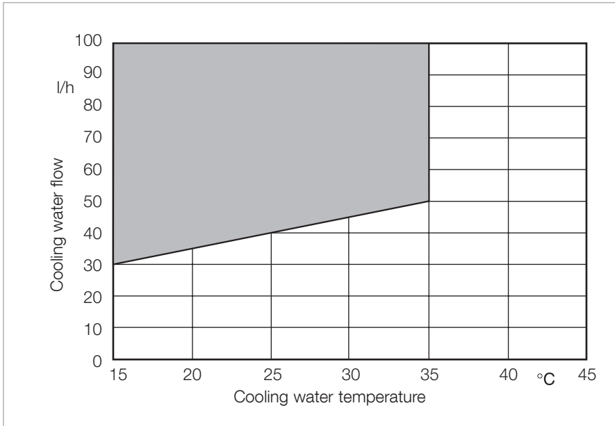
Fig. 3.12 Cooling water requirements
