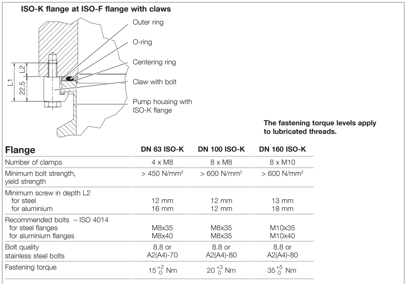
Fig. 3.7 Mounting high vacuum flange ISO-K
