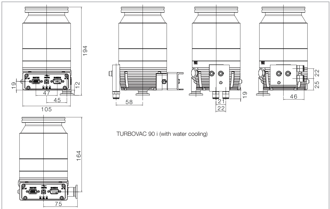
Fig. 1.10 Dimensional drawings, dimensions in mm
