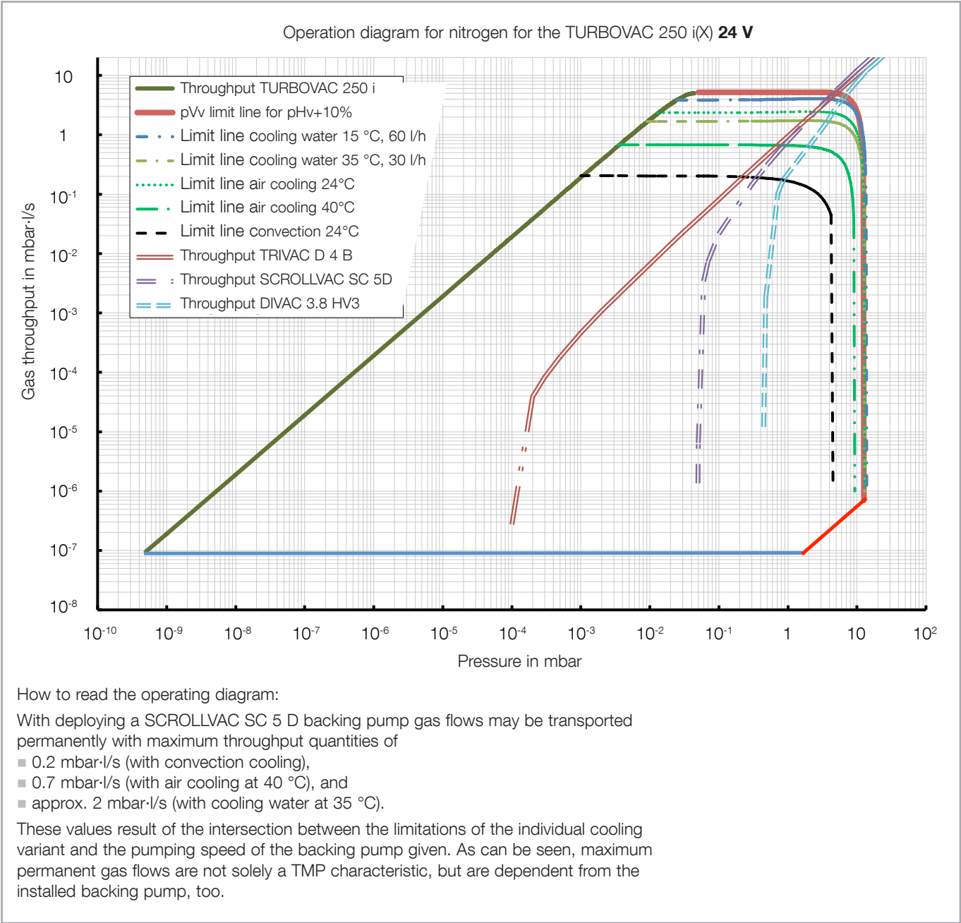
Fig. 1.6b Operation diagram for nitrogen for the TURBOVAC 250 i(X) 24 V
