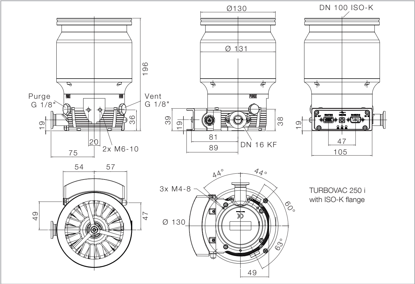
Fig. 1.15 Dimensional drawings, dimensions in mm
