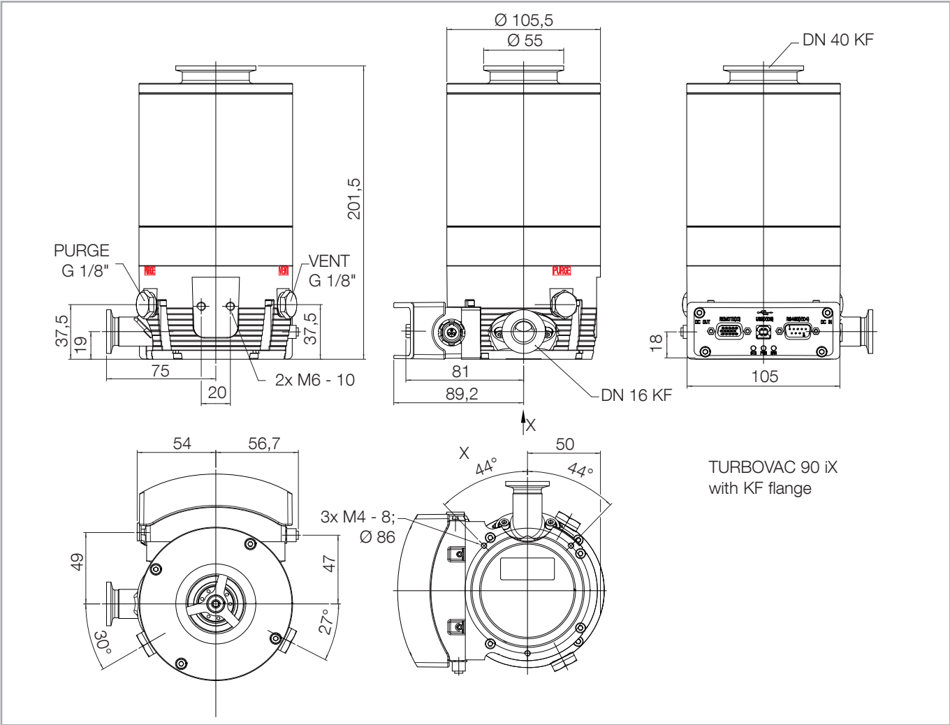
Fig. 1.14 Dimensional drawings, dimensions in mm
