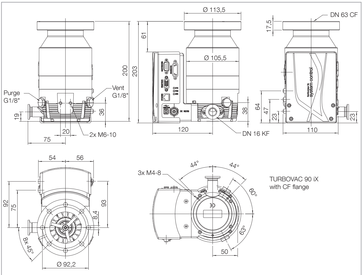
Fig. 1.13 Dimensional drawings, dimensions in mm
