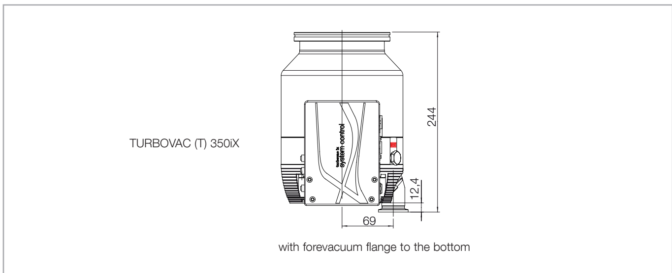
Fig. 1.29 Dimensional drawings
