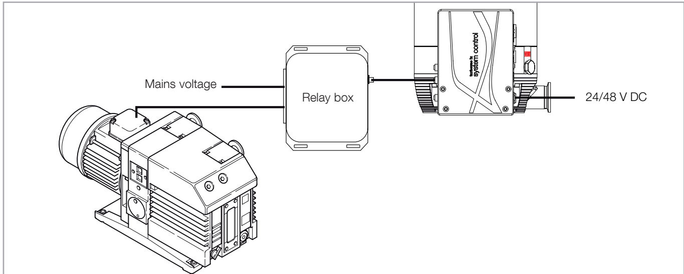
Fig. 3.9 Connecting the forevacuum pump via the relay box
