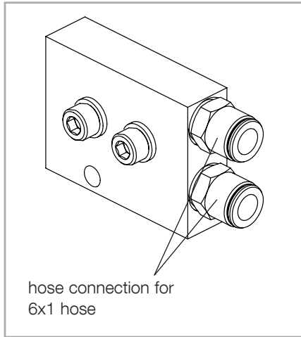
Fig. 3.11 Cooling water block
