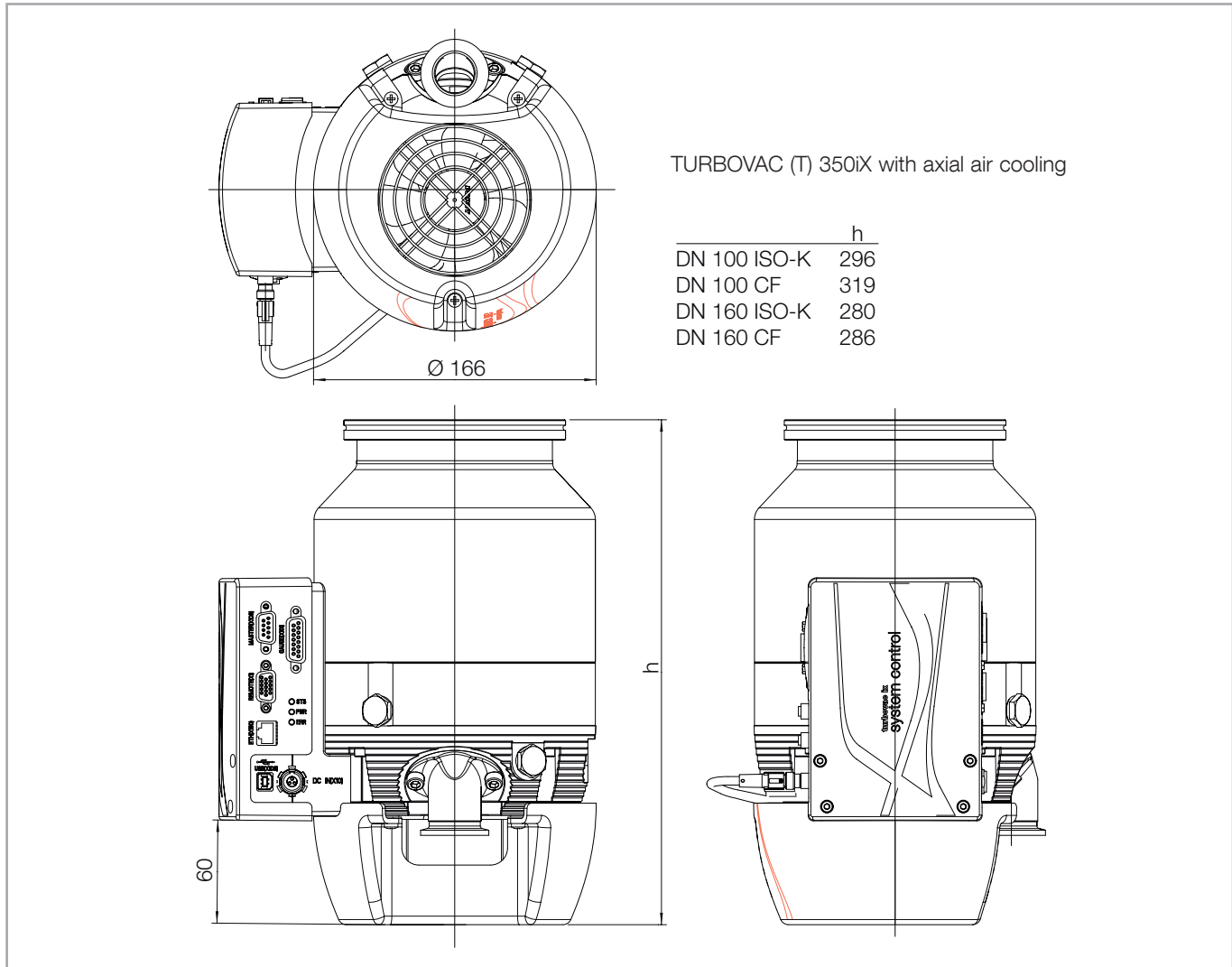
Fig. 1.28 Dimensional drawings
