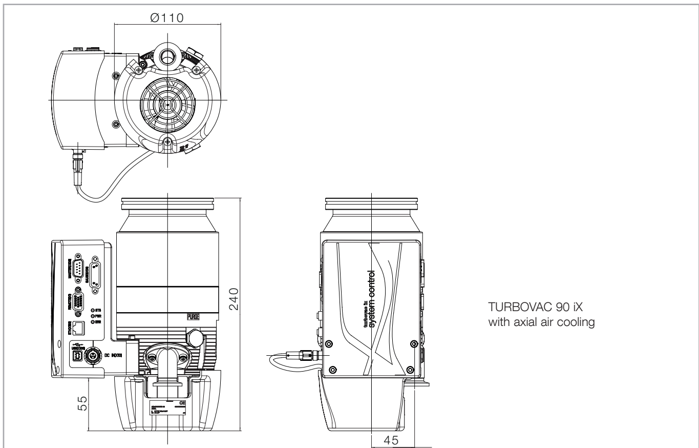
Fig. 1.12 Dimensional drawings, dimensions in mm
