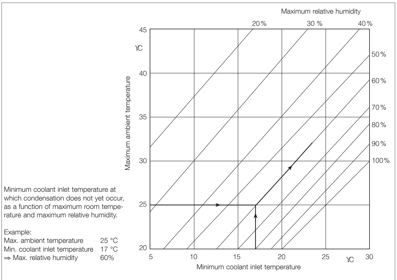
Abb. 3.13 Dewpoint diagram
