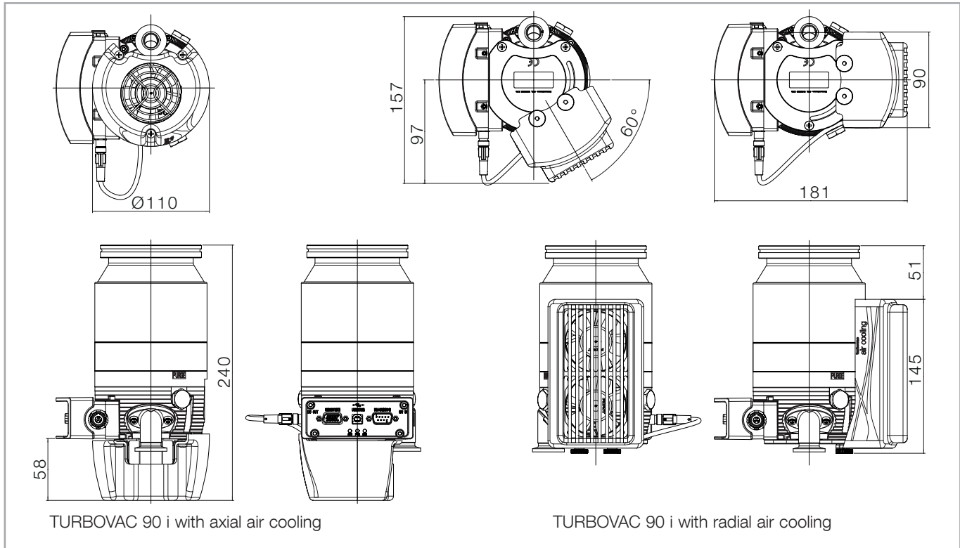
Fig. 1.11 Dimensional drawings, dimensions in mm
