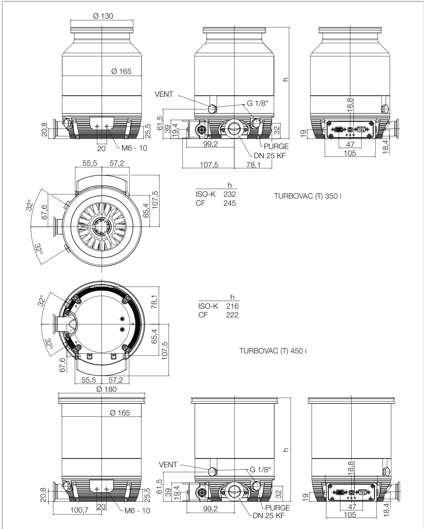
Fig. 1.20 Dimensional drawings, dimensions in mm
