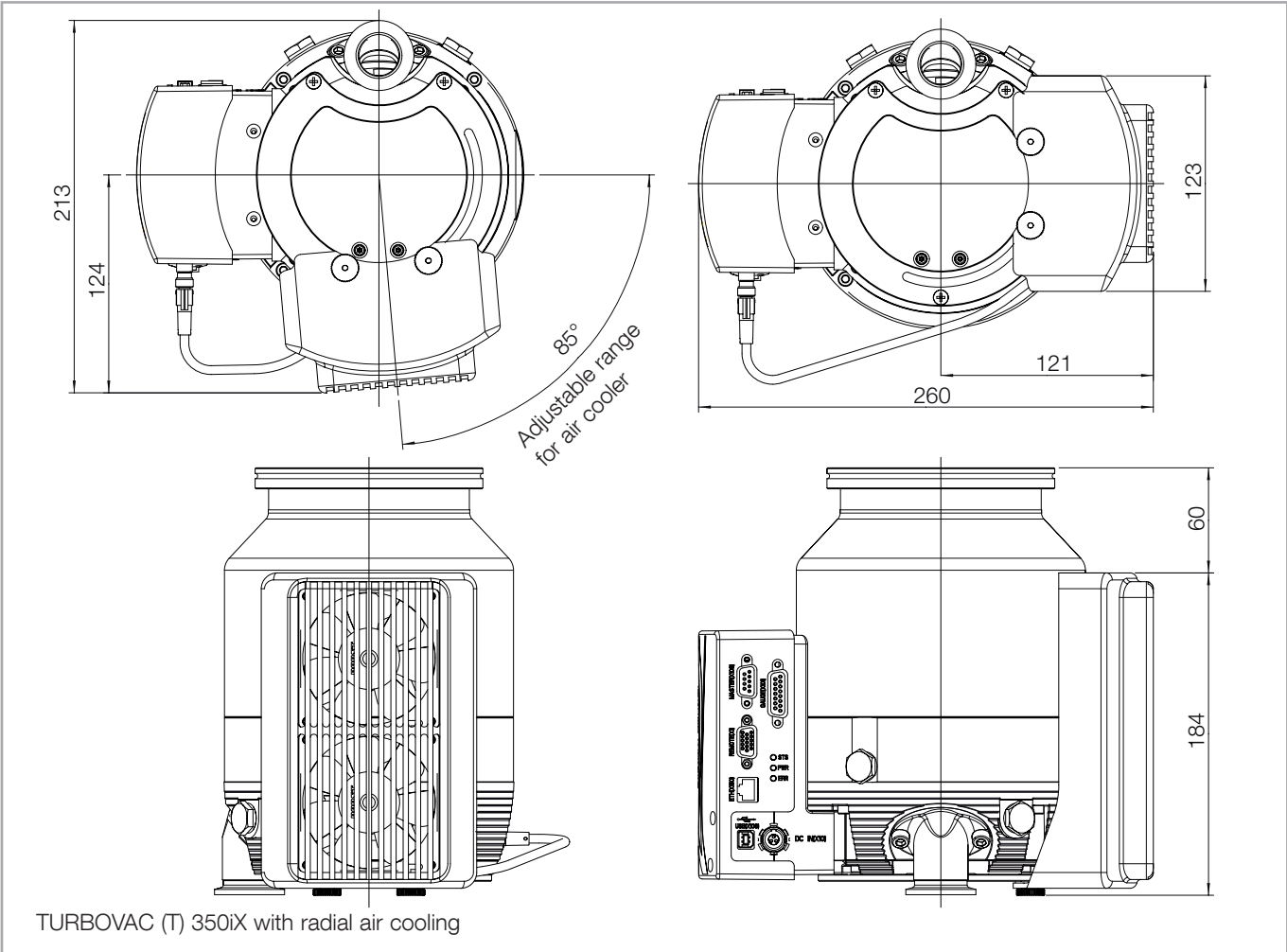
Fig. 1.25 Dimensional drawings
