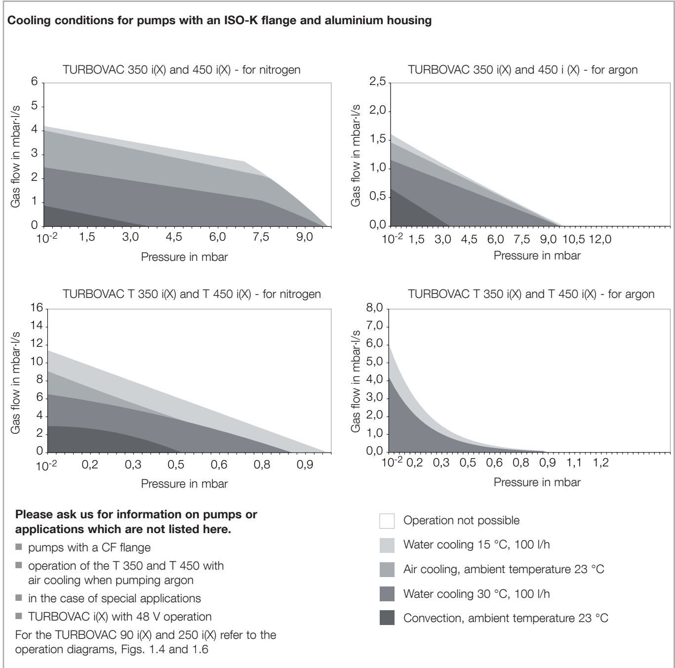
Fig. 1.9 Cooling conditions
