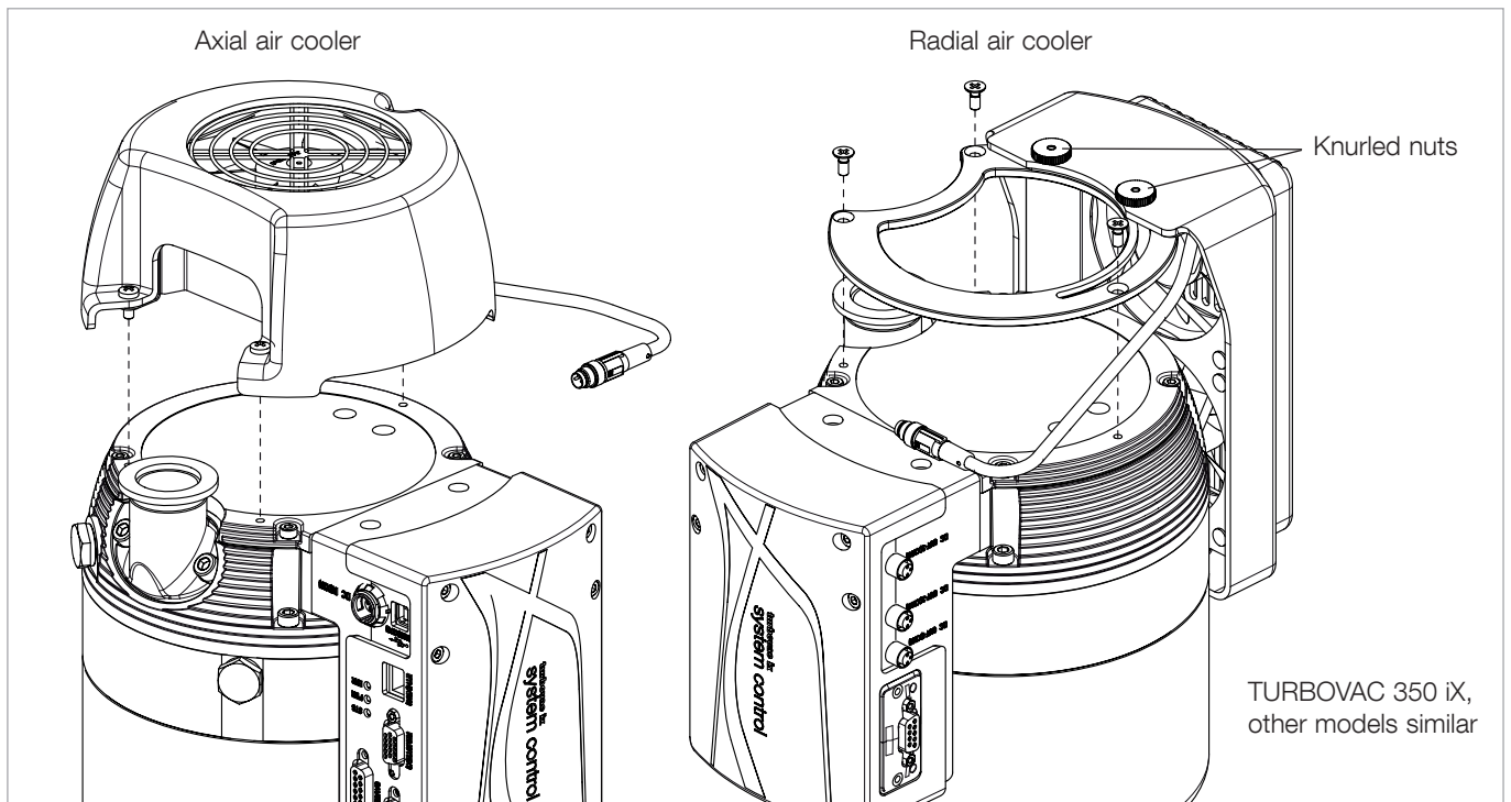
Fig. 3.10 Mounting air coolers
