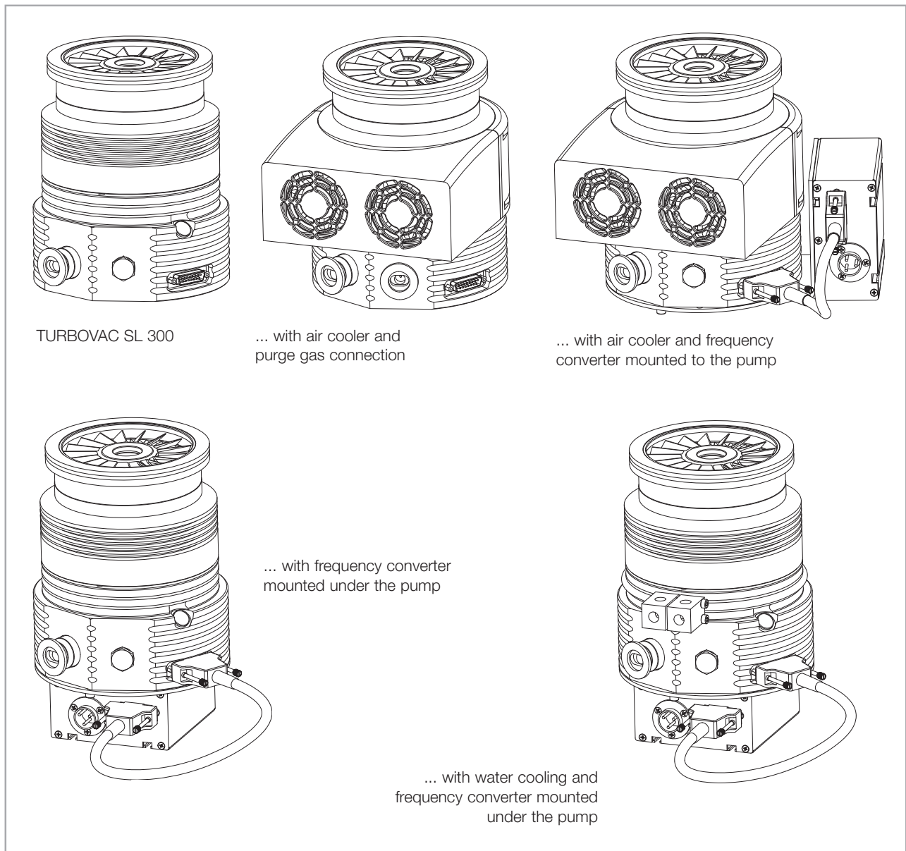
Fig. 1.1 Examples of SL 300
