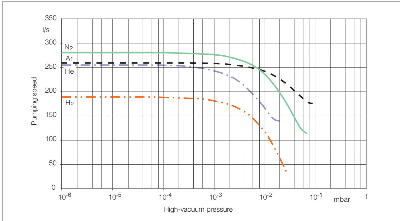
Fig. 1.2 Pumping speed curves of the SL 300
