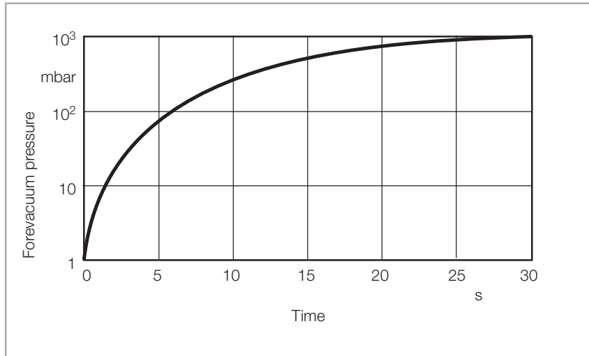
Fig. 3.6 Maximum rise in pressure
