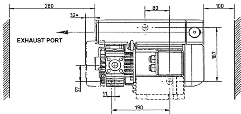
SPACE FOR EXHAUST FILTER EXCHANGE AND COOLING
