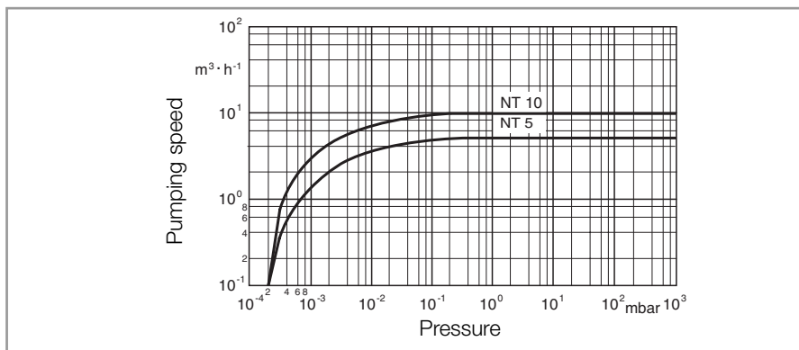
Fig. 4 Pumping speed curves of the TRIVAC NT 5 and NT 10
