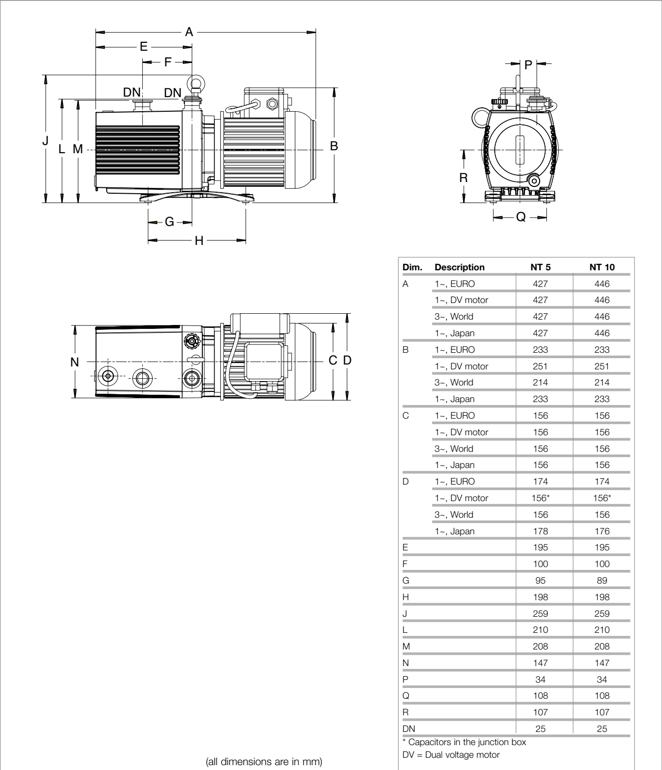
Fig. 5 Dimensional drawing
