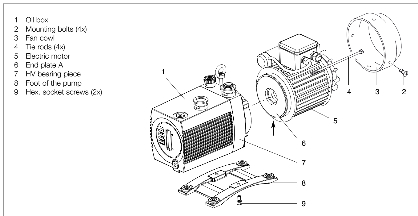
Fig. 10 Disassembly and assembly of the electric motor
