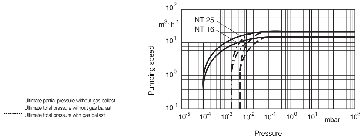
Fig. 1.5 Pumping speed characteristics of the TRIVAC NT 16 / NT 25
