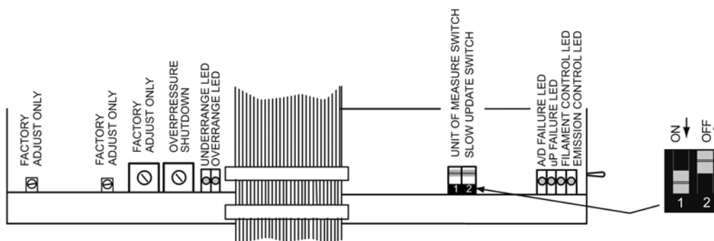
Figure 4-1 Ion Gauge Electrometer Module Top View
