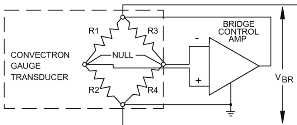
Figure 5-13 Convectron Gauge Schematic
