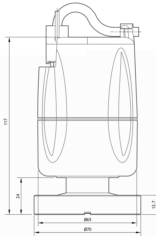
Figure 3 - Dimensions (mm) of the nWRG-DN40 CF
