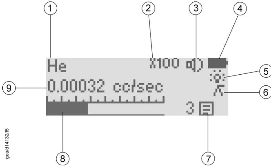
Figure 5 - Running screen
