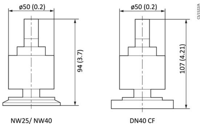
Figure 1 Dimensions
