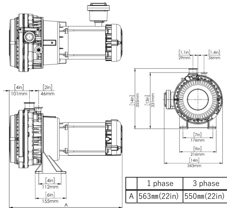
ISP-500C Dimension
